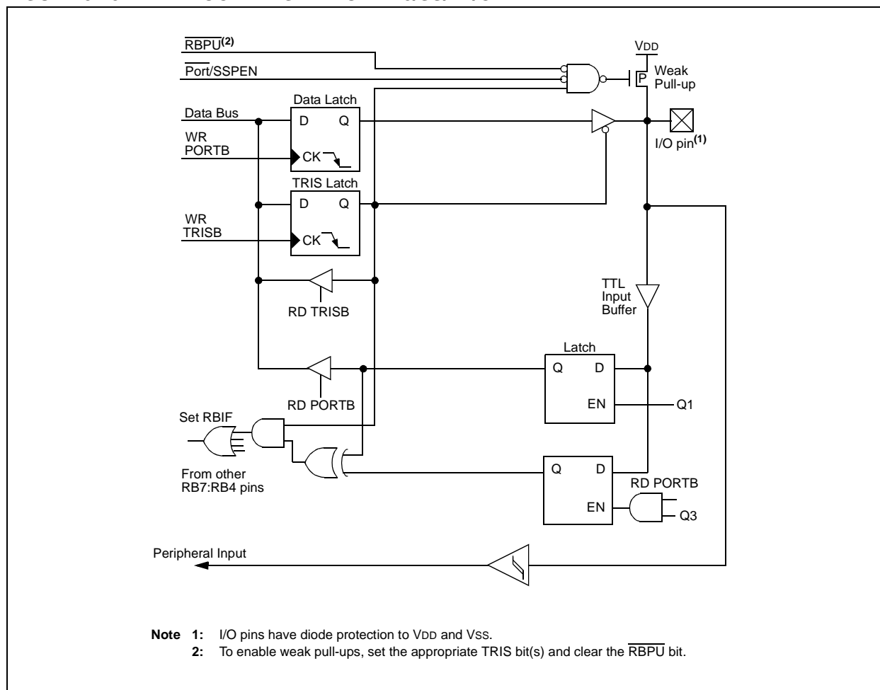
FIGURE 5-13: BLOCK DIAGRAM OF RB5/ \overline{\text{SS}} /TX/CK PIN
